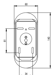
WALL BRACKET*
